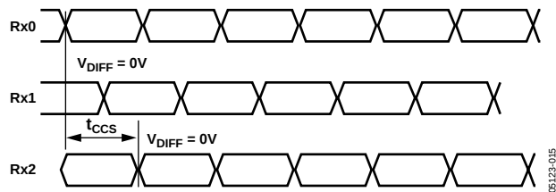
Figure 15. Channel-to-Channel Skew Timing
