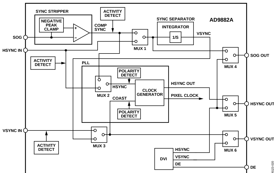
Figure 20. Sync Processing Block Diagram
