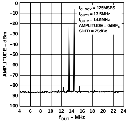
Figure 15. Two-Tone SFDR
