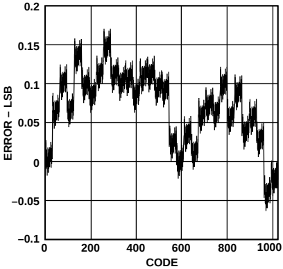
Figure 12. Typical INL
