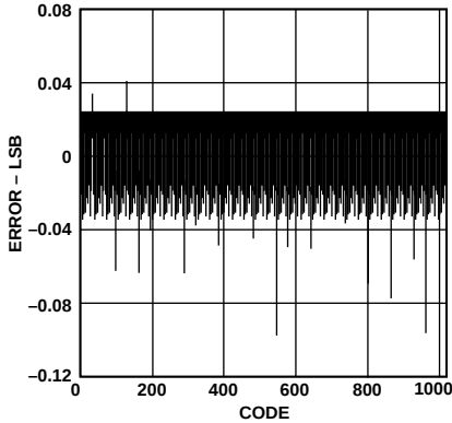
Figure 13. Typical DNL
