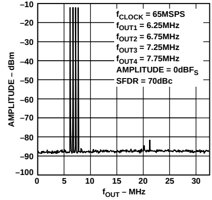
Figure 16. Four-Tone SFDR
