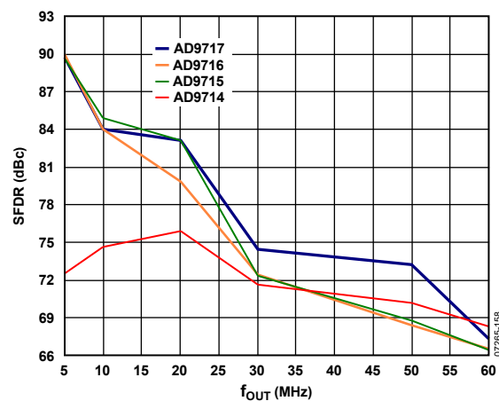
Figure 58. AD9714/AD9715/AD9716/AD9717 SFDR at 3.3 V
