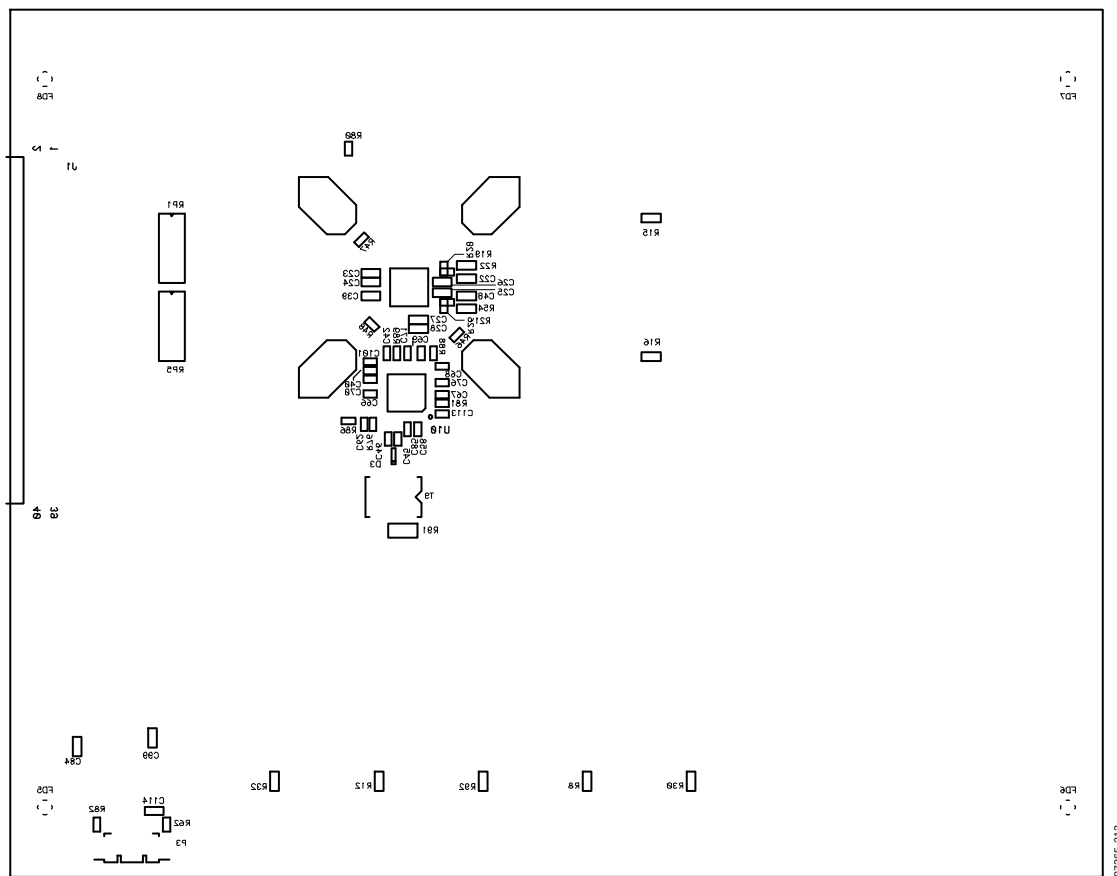
Figure 130. Silkscreen—Secondary Side
