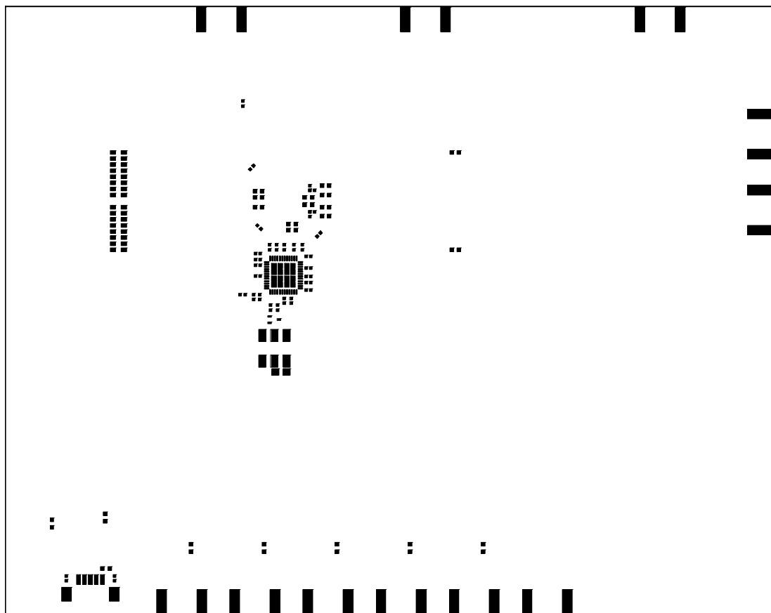
Figure 128. Secondary Side Paste
