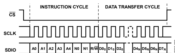
Figure 87. Serial Register Interface Timing, LSB First Write
