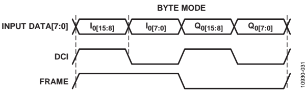
Figure 34. Timing Diagram for Byte Mode
