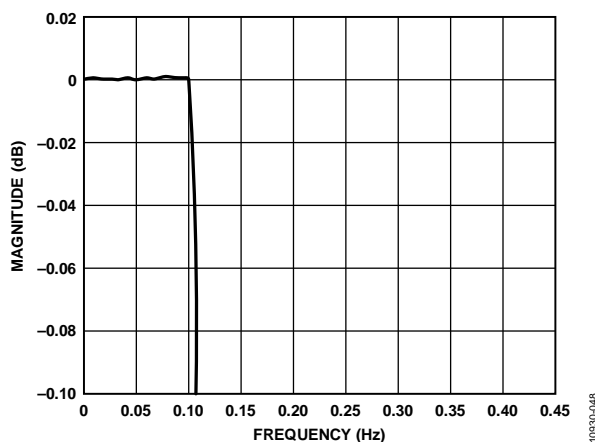
Figure 43. Pass-Band Detail of 8× Mode
