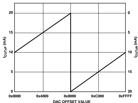
Figure 46. DAC Output Currents vs. DAC Offset Value
