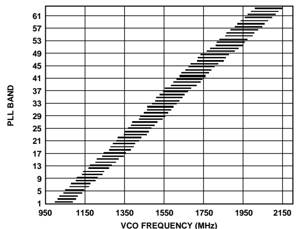
Figure 53. PLL Lock Range for a Typical Device
