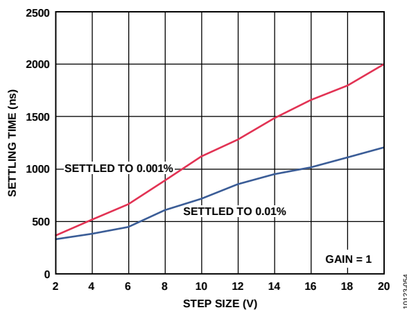
Figure 51. Settling Time vs. Step Size ( G = 1 ), R_L = 2 k \Omega , C_L = 100 pF
