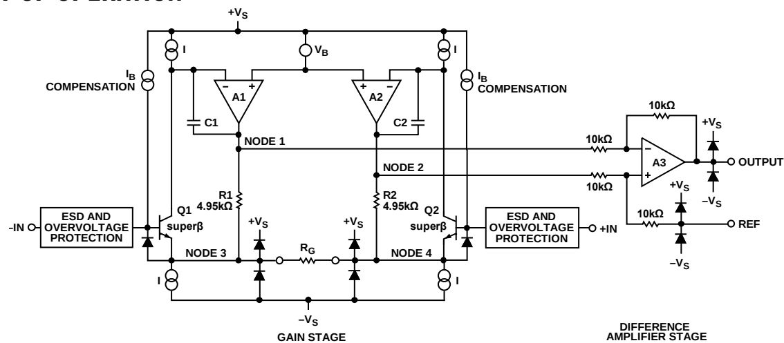
Figure 62. Simplified Schematic
