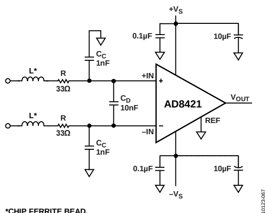
Figure 69. RFI Suppression
