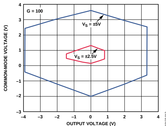
Figure 14. Input Common-Mode Voltage vs. Output Voltage; V_S = \pm 2.5\text{ V} and \pm 5\text{ V} ( G = 100 )
