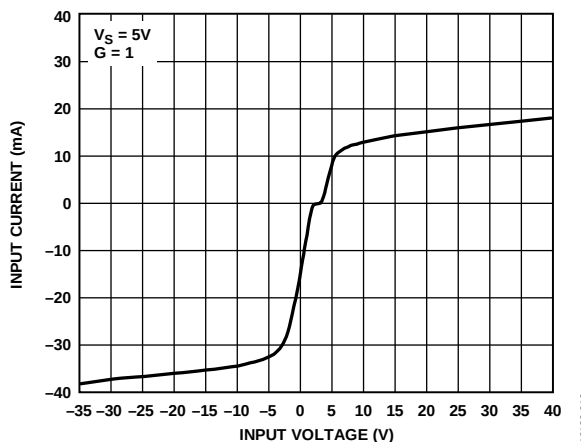
Figure 15. Input Overvoltage Performance; G = 1 , +V_S = 5\text{ V} , -V_S = 0\text{ V}
