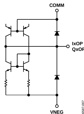
Figure 8. Output Drivers
