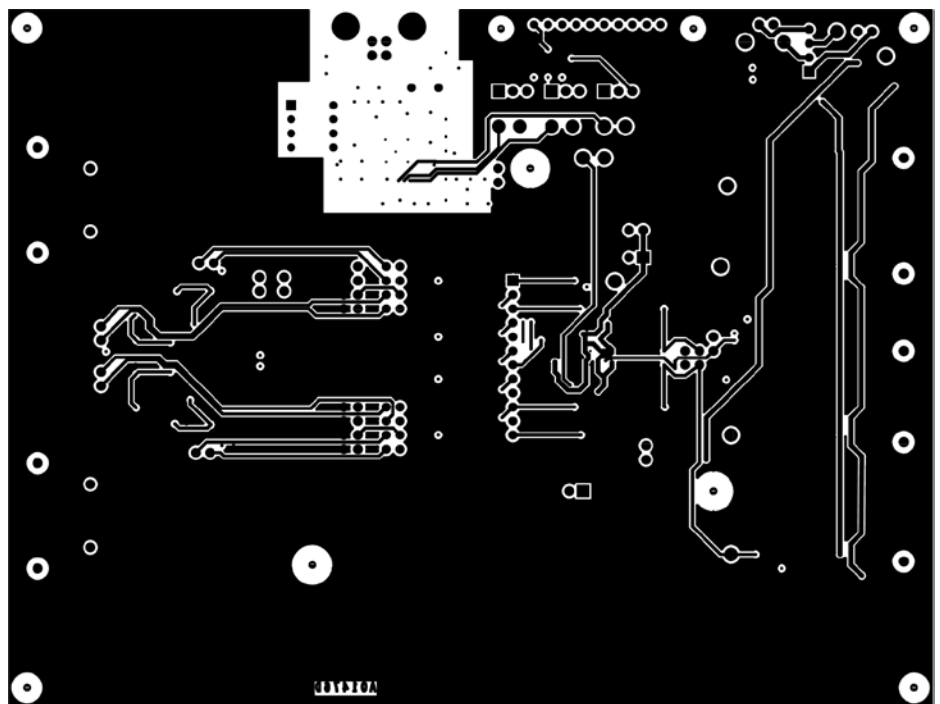
Figure 67. AD8339-EVALZ Wiring Side Copper
