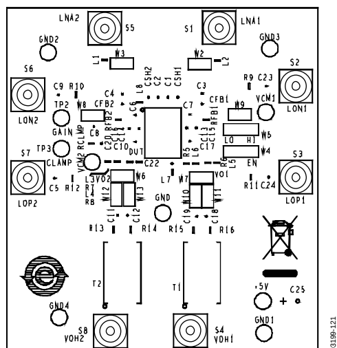
Figure 107. AD8332-EVALZ Assembly
