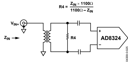
Figure 25. Single-to-Differential Circuit
