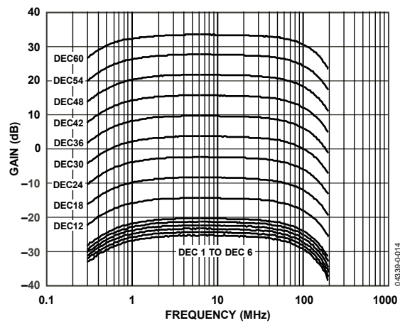
Figure 14. AC Response
