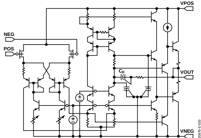
Figure 32. Simplified Schematic
