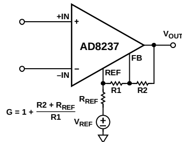
Figure 71. Calculating Gain with Reference Resistance
