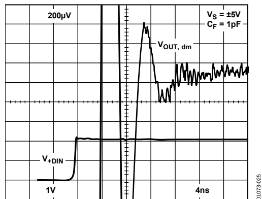
Figure 25. Settling Time
