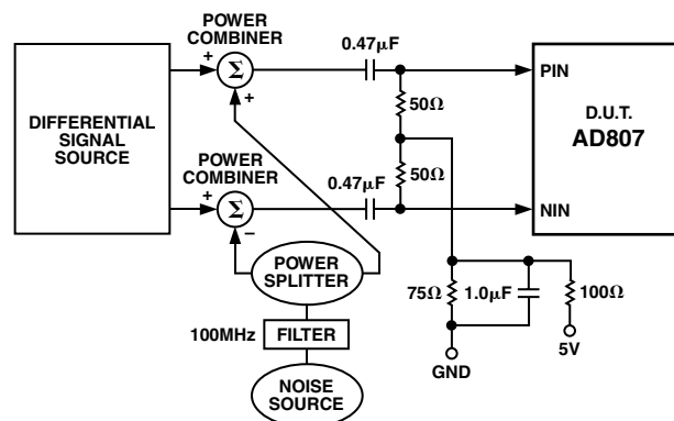
Figure 4. Bit Error Rate vs. Signal-to-Noise Ratio Test: Block Diagram
