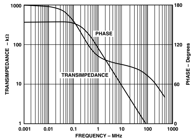
TPC 28. Open-Loop Transimpedance and Phase vs. Frequency
