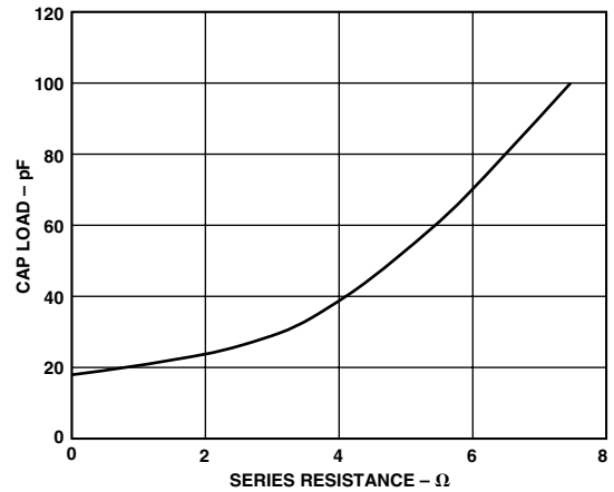
TPC 26. R_S and C_L vs. 30% Overshoot
