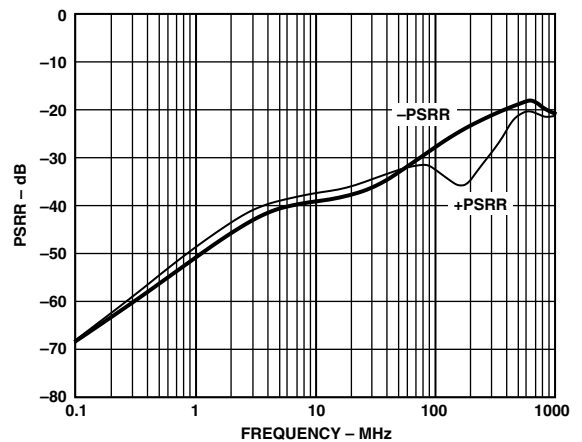
TPC 27. PSRR vs. Frequency; V_S = \pm 6\text{ V} or V_S = \pm 2.5\text{ V}
