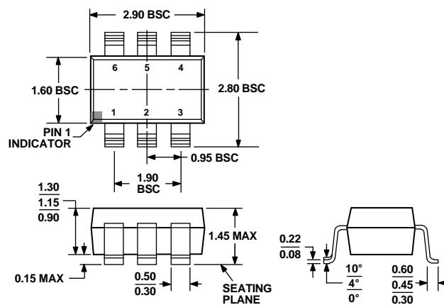
Figure 30. 6-Lead Small Outline Transistor Package [SOT-23] (RJ-6) Dimensions shown in millimeters
