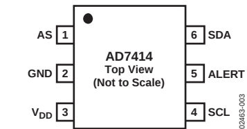
Figure 3. AD7414 Pin Configuration (SOT-23)
