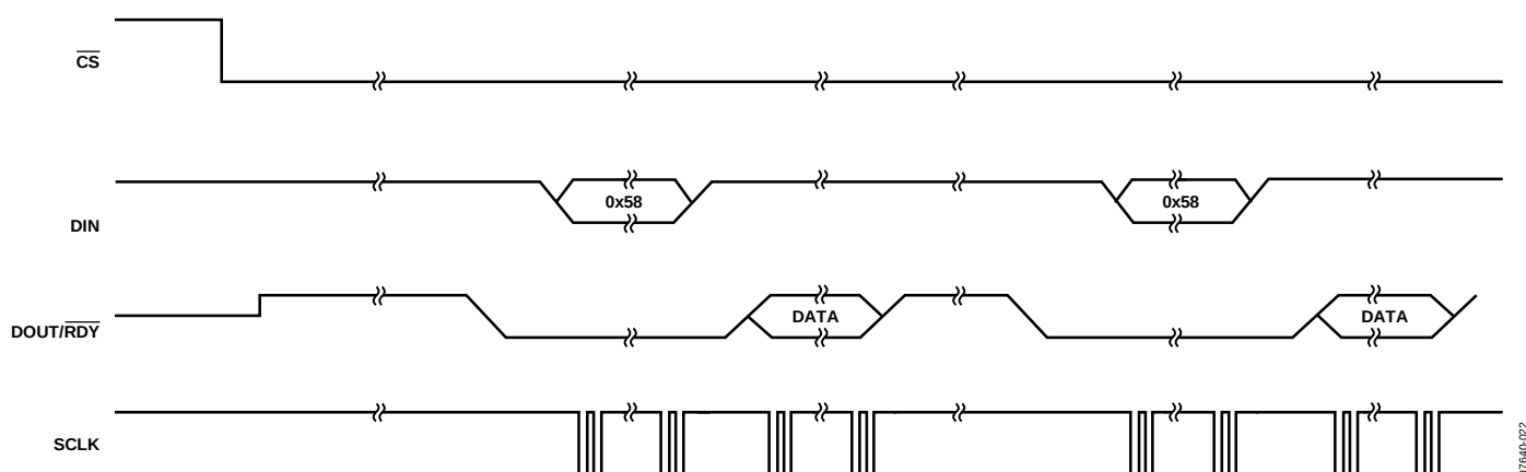
Figure 30. Continuous Conversion
