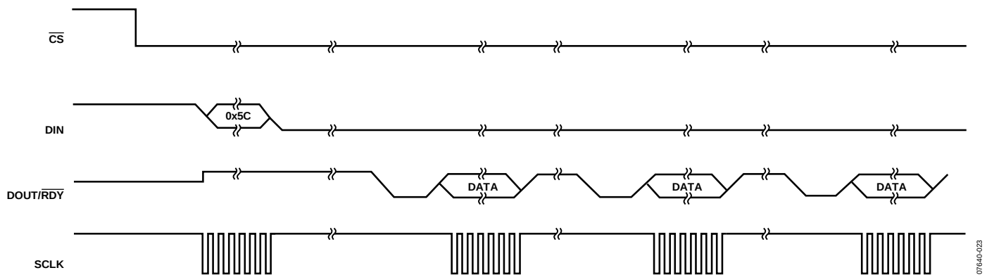
Figure 31. Continuous Read
