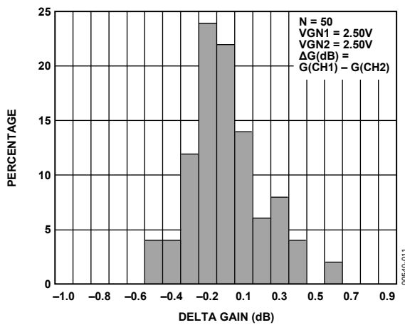
Figure 11. Gain Match; VGN1 = VGN2 = 2.50 V
