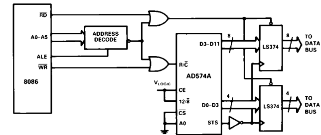
Figure 13. 8086 Stand-Alone Configuration
