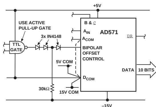
Figure 5. Bipolar Offset Controlled by Logic Gate Gate Output = 1: Unipolar 0 V–10 V Input Range Gate Output = 0: Bipolar \pm 5 V Input Range
