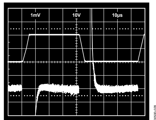
Figure 27. Settling Time, Gain = 100
