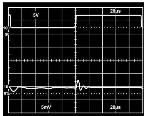
Figure 27. Load Transient Response (0 mA to –1 mA Load)
