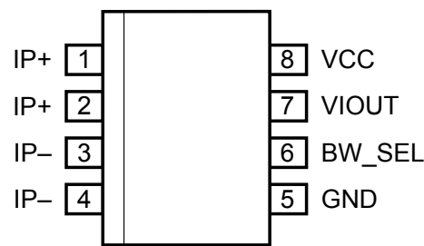
Pinout Diagram
