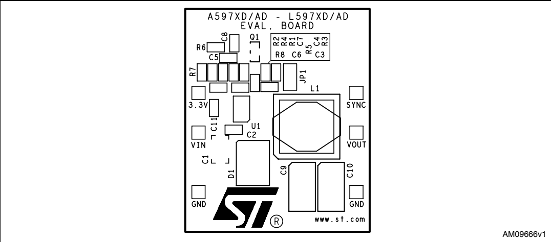
Figure 22. PCB layout (component side)
