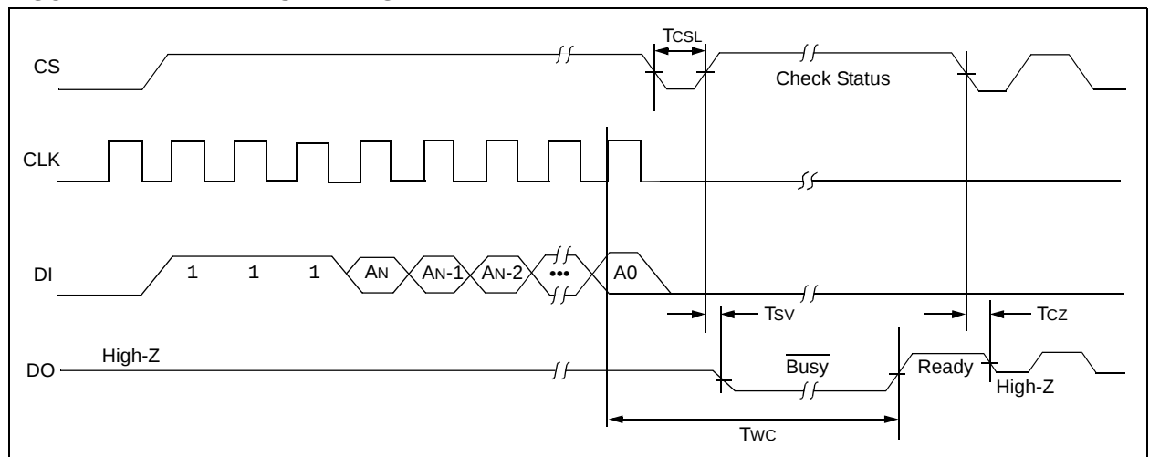
FIGURE 2-1: ERASE TIMING
