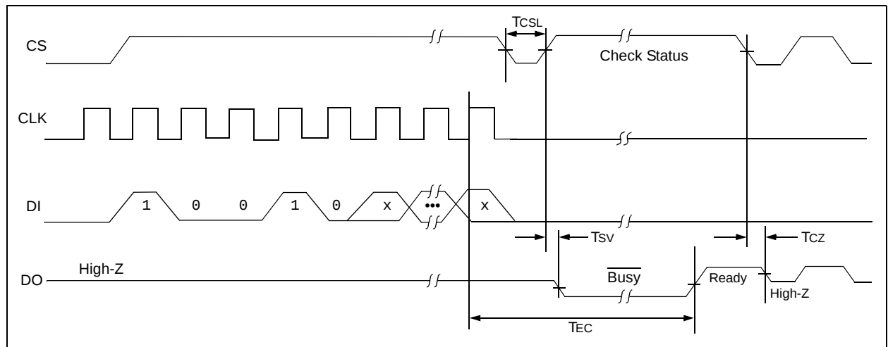
FIGURE 2-2: ERAL TIMING
