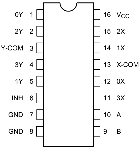
74VHC4052AFT
