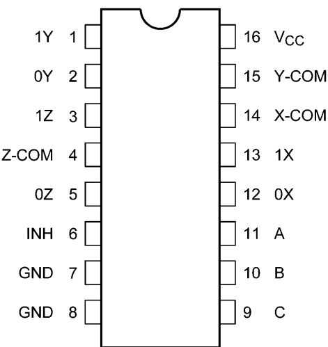
74VHC4053AFT
