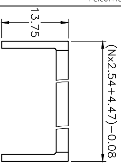
LOW PROFILE STRAIN RELIEF
