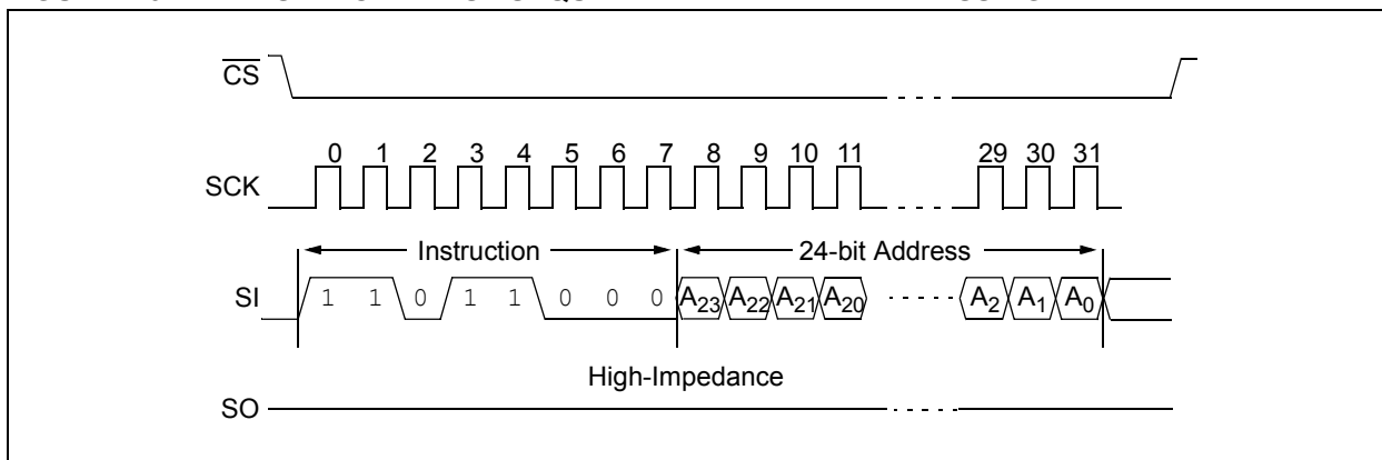
FIGURE 2-9A: SECTOR ERASE SEQUENCE WITH 24-BIT ADDRESSING
