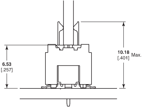
Vertical Plug with Right Angle Receptacle
