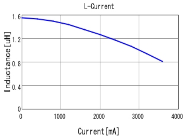
■ 1269AS-H-1R5M L-Current 20degC
