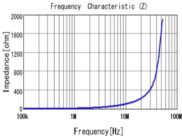
■ 1269AS-H-1R5M |Z|
