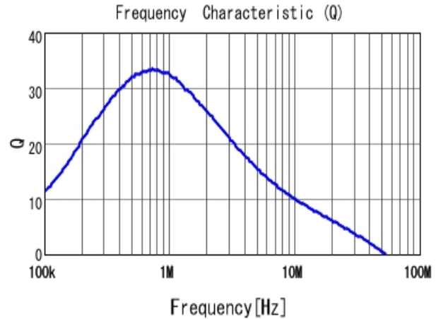
■ 1269AS-H-1R5M Q
