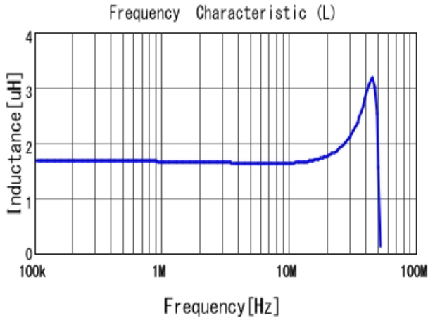
■ 1269AS-H-1R5M L
