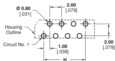
Recommended PCB Layout 1.60 [063] Thickness (For Even Position Connectors)
