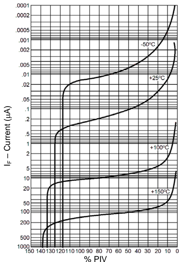
FIGURE 1 Typical Reverse Current vs. PIV
