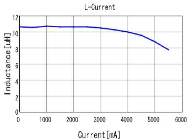
■ 1217AS-H-100M L-Current 20degC
