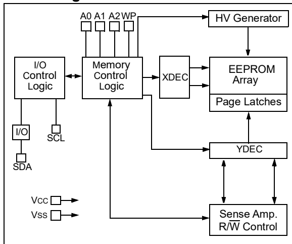
Block Diagram
