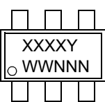
6-Lead SOT-23
