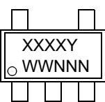
5-Lead SOT-23
