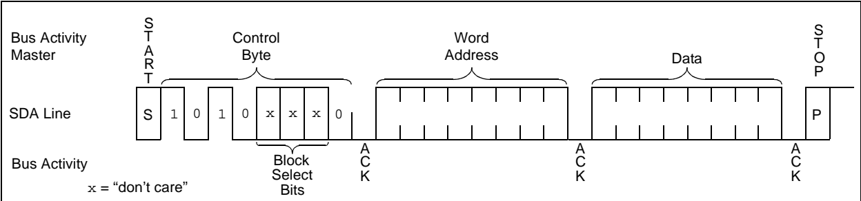
FIGURE 5-1: BYTE WRITE
