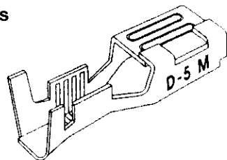
Receptacle Contact (Used in Receptacle Housing)
