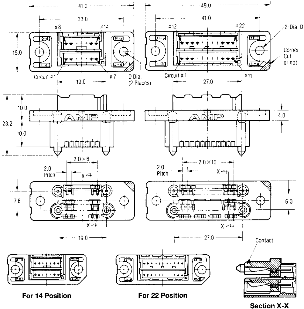
For 14 Position Panel Cutout (connector mounting side)
