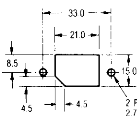
Movable Side
