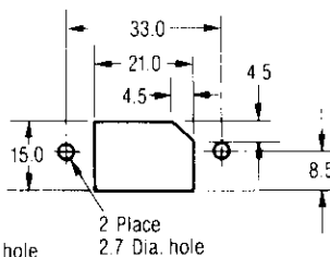
Fixed Side
