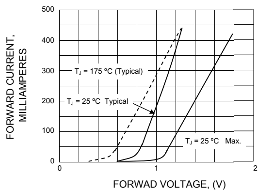
FIG.2 - FORWARD CURRENT AS A FUNCTION FORWARD VOLTAGE
