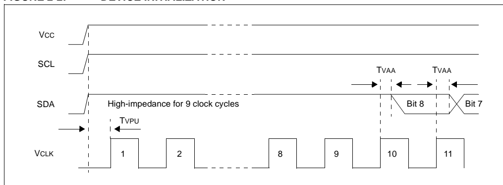
FIGURE 2-2: DEVICE INITIALIZATION
