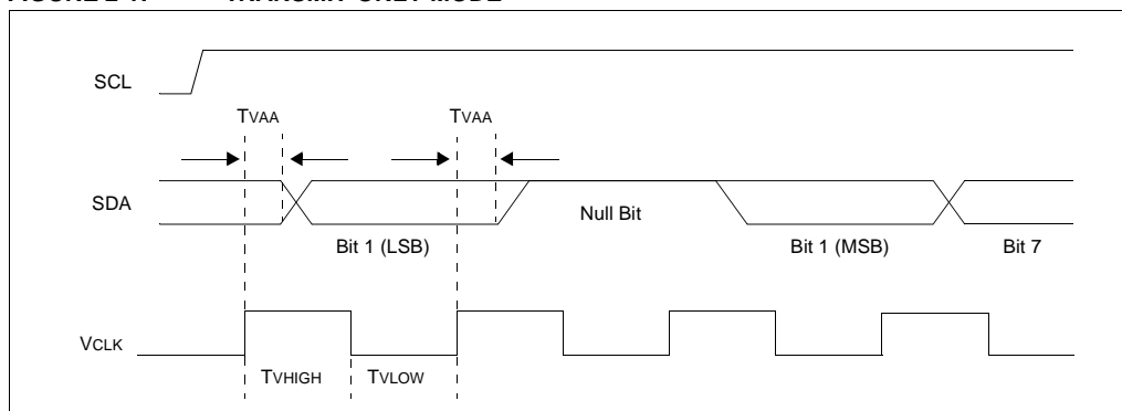
FIGURE 2-1: TRANSMIT-ONLY MODE
