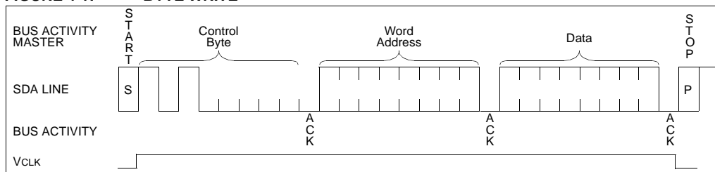
FIGURE 4-2: BYTE WRITE
