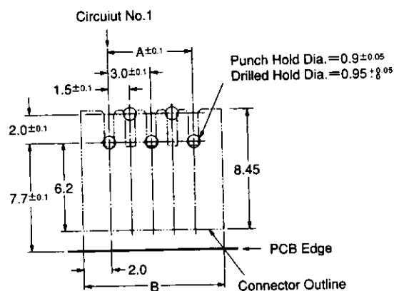
PC Board Layout (Component Side) (Applicable board thickness=1.6mm)
