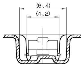
SECT. F-F
