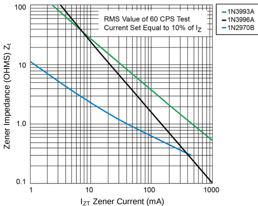
FIGURE 3 Typical Zener Impedance vs Zener Current for Types Shown
