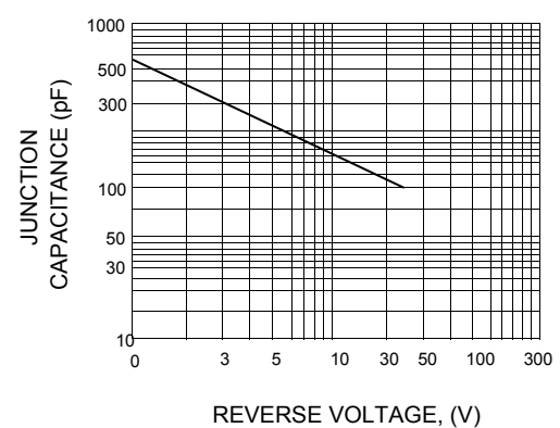
FIG. 4 - TYPICAL JUNCTION CAPACITANCE PER LEG
