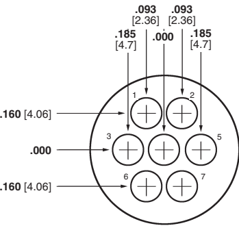
Arrangement 13-7 Max. Wire Ins. Dia. = .100 [2.54]
