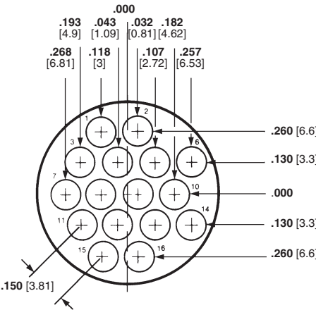
Arrangement 17-16 Max. Wire Ins. Dia. = .100 [2.54]
