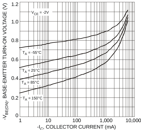
Fig. 5 Typical Base-Emittor Turn-On Voltage vs. Collector Current
