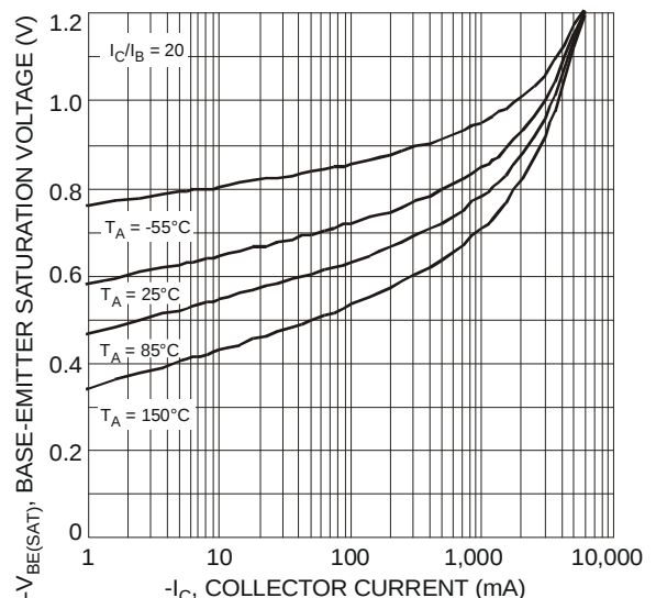
Fig. 6 Typical Base-Emittor Saturation Voltage vs. Collector Current
