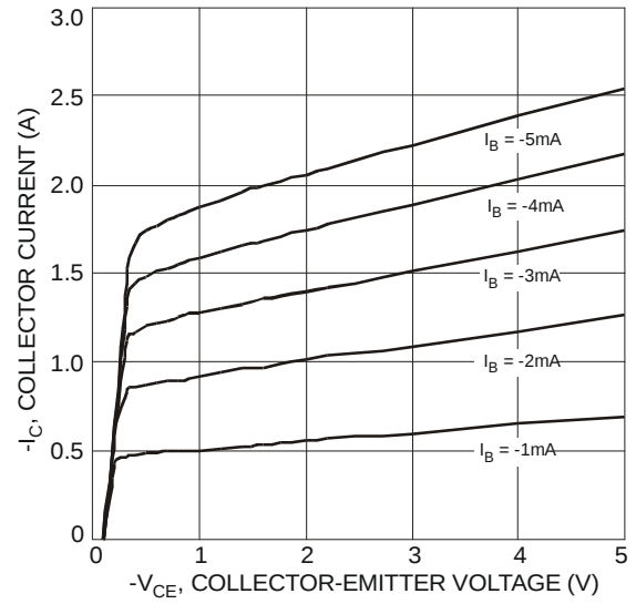
Fig. 2 Typical Collector Current vs. Collector-Emittor Voltage
