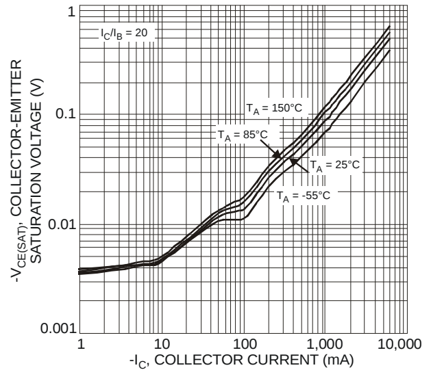
Fig. 4 Typical Collector-Emittor Saturation Voltage vs. Collector Current
