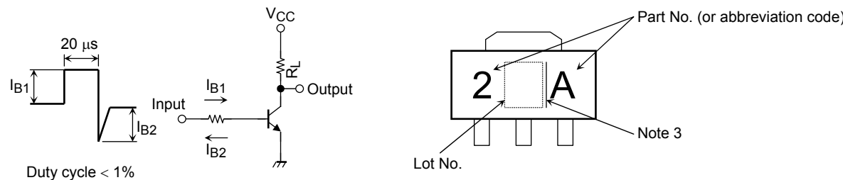
Figure 1 Switching Time Test Circuit & Timing Chart
