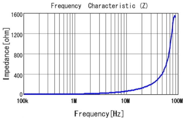
1285AS-H-1R0M |Z|
