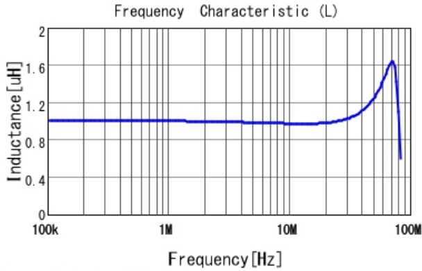
1285AS-H-1R0M L
