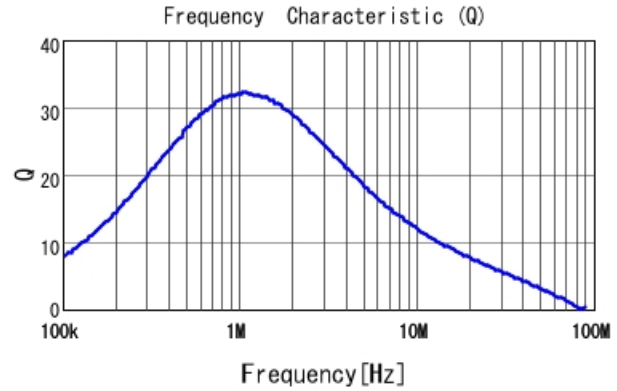
1285AS-H-1R0M Q
