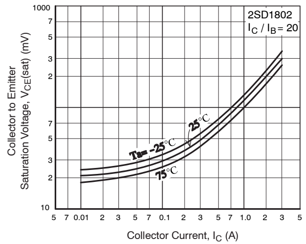
Figure 14. V_{CE(sat)} - I_C
