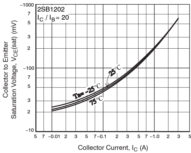
Figure 13. V_{CE(sat)} - I_C
