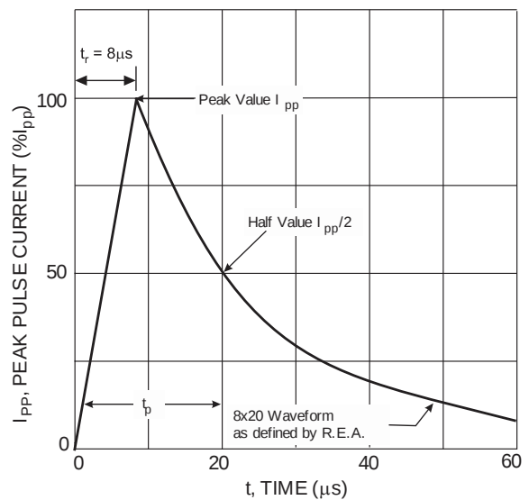
Figure 8 Pulse Waveform
