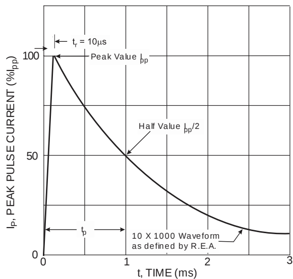
Figure 9 Pulse Waveform
