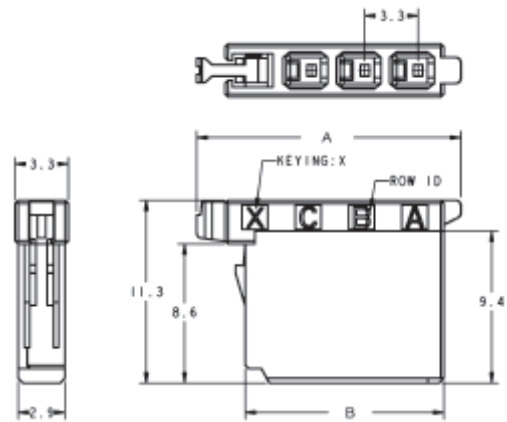
Horizontal/Vertical Type
