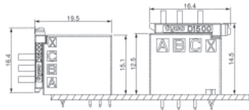
Horizontal/Vertical Type
